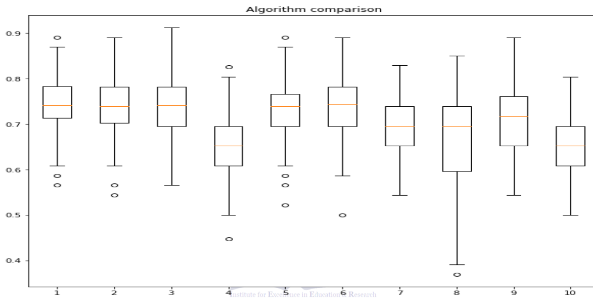
Figure 1: Algorithm Comparison
