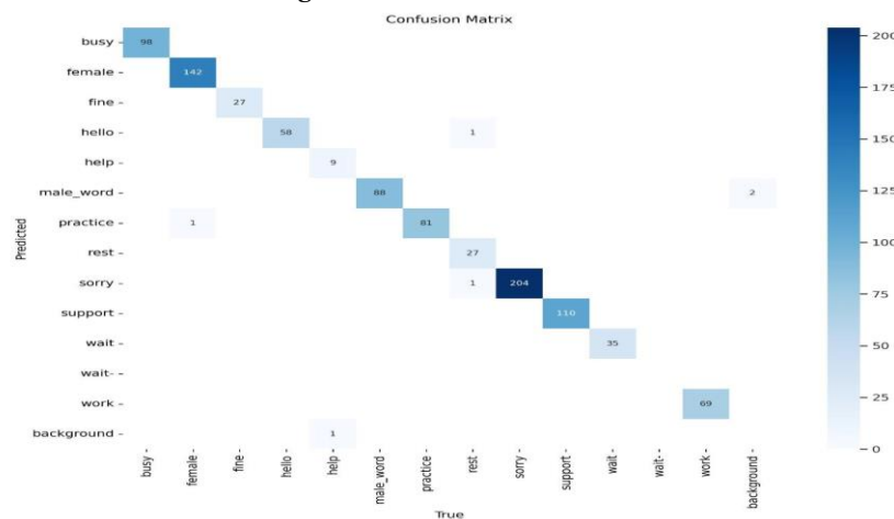
Figure 5.3 Confusion Matrix
