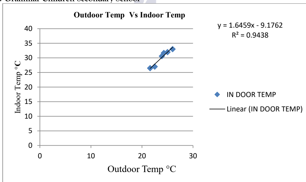
Chart 2a: Correlation of Outdoor and Indoor Temperature in New Grammar Children High School in winter.
