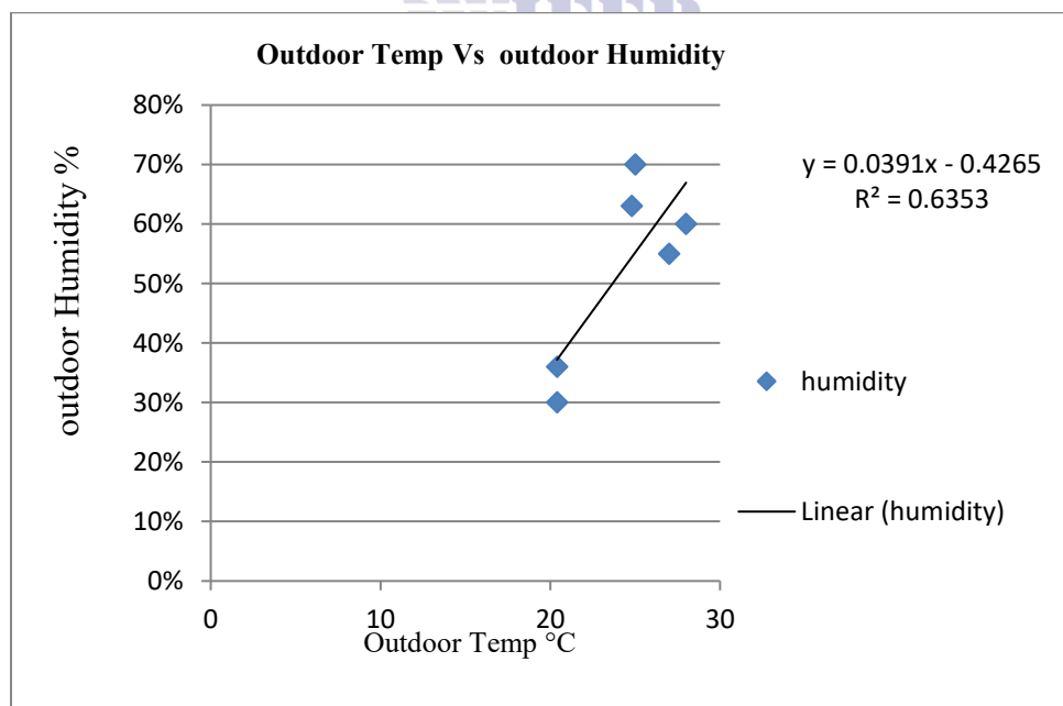
Chart 1b: Correlation of Outdoor Temperature and Outdoor Humidity in Al Rehman School in winter.
